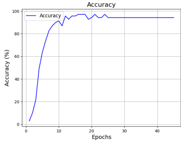
Gambar 6. Hasil accuracy
