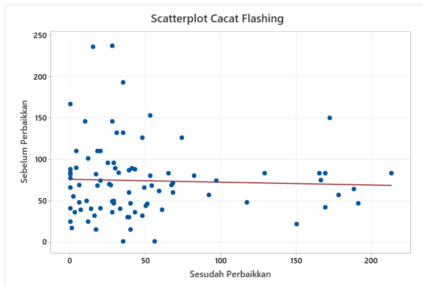
Gambar 3.15. Diagram scatter cacat flashing
