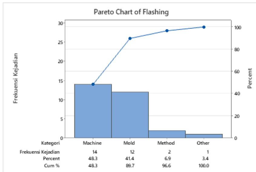
Gambar 3.11. Diagram pareto cacat flashing
