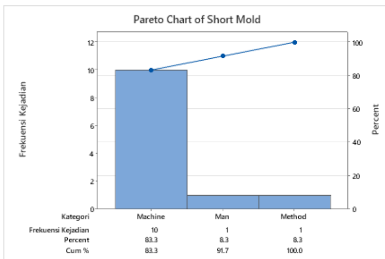
Gambar 3.9. Diagram pareto cacat short mold
