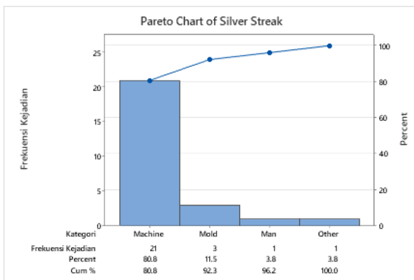
Gambar 3.10. Diagram pareto cacat silver streak
